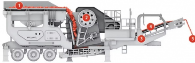
1. Vibrating feeder 2. Jaw crusher 3. Heavy duty rock 4. Discharging belt conveyor
